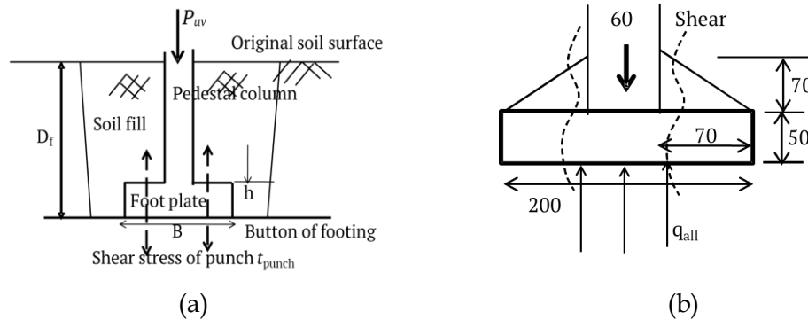
Figure 4. A practical design of foundation in this study: (a) Designed in the contractual, (b) Modified footing structure
