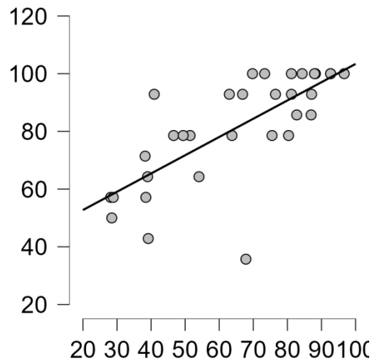
Gambar 1. Plot Korelasi
