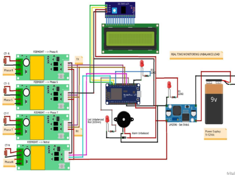
Figure 2 Diagram of real time the current unbalance monitoring with Arduino-based
