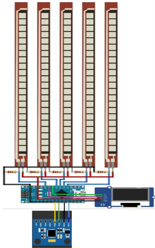
Figure 2. Whole circuit
