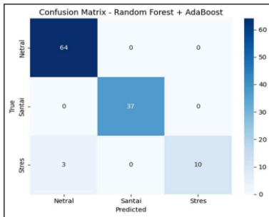
Figure 14. Confusion Matrix Plot Results of Ensemble Model (Random Forest + AdaBoost) in EEG Signal Classification to Determine Stress Levels
