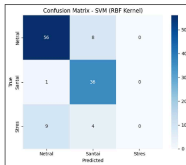
Figure 10. Confusion Matrix Plot Results of a Support Vector Machine Model in EEG Signal Classification to Determine Stress Levels
