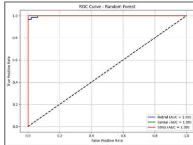
Figure 13. Random Forest Model Receiver Operating Characteristics (ROC) Graphic Results
