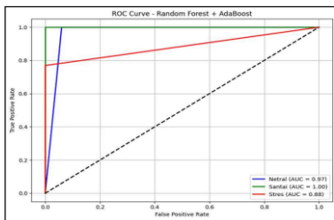
Figure 15. Receiver Operating Characteristics (ROC) Chart Results for Ensemble Model (Random Forest + AdaBoost)
