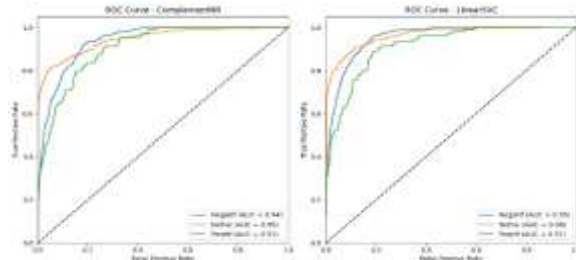
Figure 5. ROC Curve of Naïve Bayes & SVM (Linear SVC)
