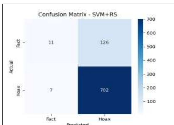
Figure 3. Confusion Matrix Plot Support Vector Machine Algorithm Based on Randomized Search Optimization
