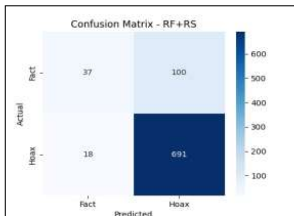
Figure 5. Confusion Matrix Plot Random Forest Algorithm Based on Randomized Search Optimization
