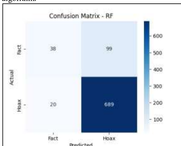
Figure 4. Confusion Matrix Plot Random Forest Algorithm
