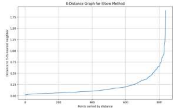
Figure 1 K-Distance Graph for Elbow Method
