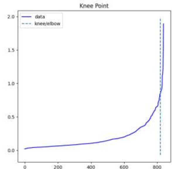
Figure 2 K-Distance Graph for Elbow Method Using KneeLocator
