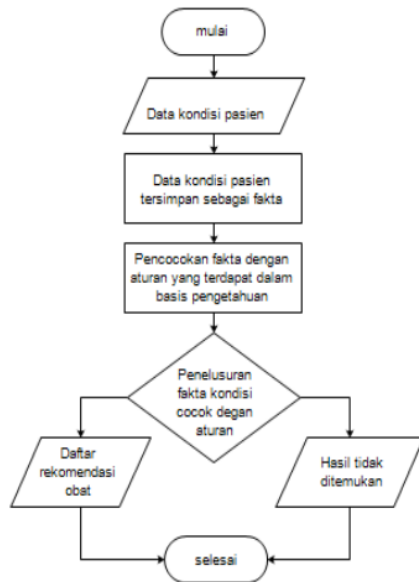
Gambar 1. Proses penelusuran fakta
