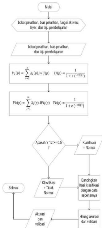
Gambar 3. Flowchart Testing Jaringan Saraf Tiruan Backpropagation
