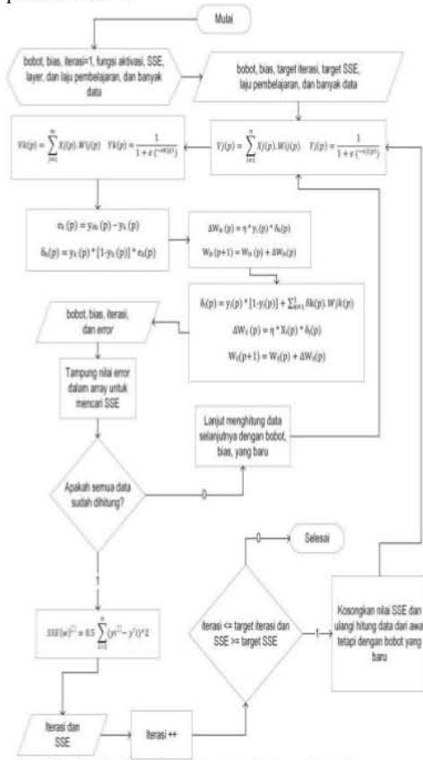
Gambar 2. Flowchart Training Jaringan Saraf Tiruan Backpropagation
