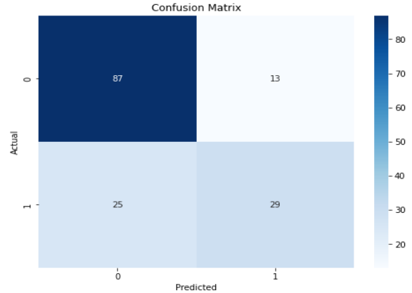
Figure 4. confusion matrix with the highest accuracy
