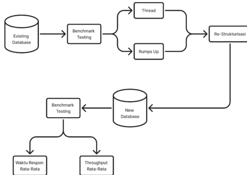
Gambar 1 Database Testing Flow
