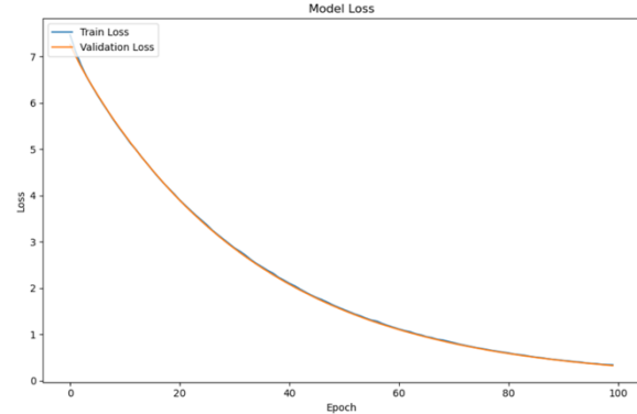
Figure 13. Training and Validation Loss Graph of the Wrist Model Using the Dataset by Malik et al.
