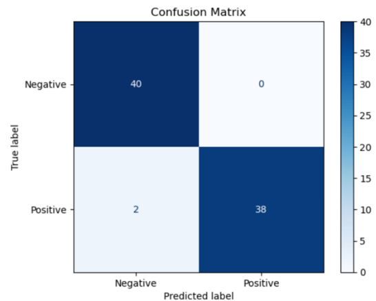
Figure 14. Confusion Matrix for Wrist Model Using the Dataset by Malik et al.
