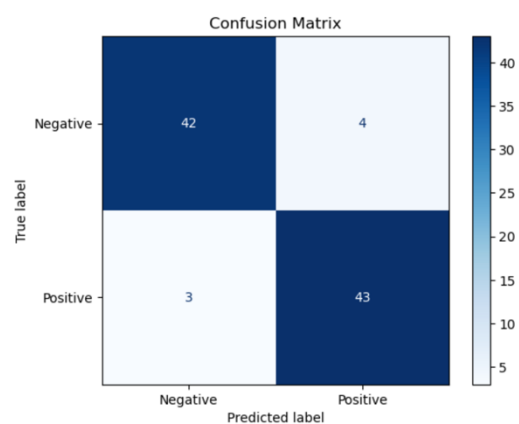
Figure 17. Confusion Matrix Results of the Hand Model
