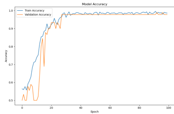
Figure 15. Training and Validation Accuracy Graph of the Hand Model
