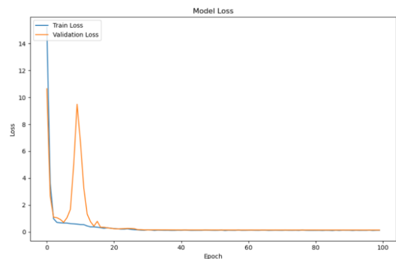
Figure 16. Training and Validation Loss Graph of the Hand Model
