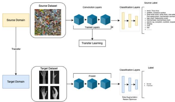
Figure 7. Phases of the Transfer Learning Process for Bone Fracture Classification
