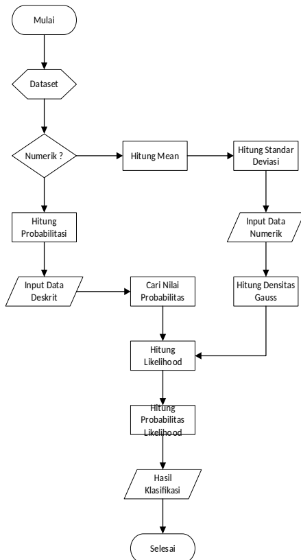
Gambar 5. Flowchart Naive Bayes
