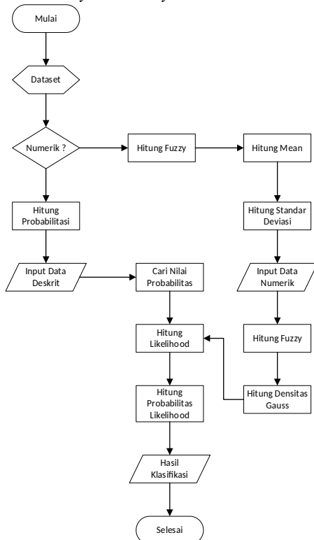
Gambar 6. Flowchart Fuzzy Naive Bayes
