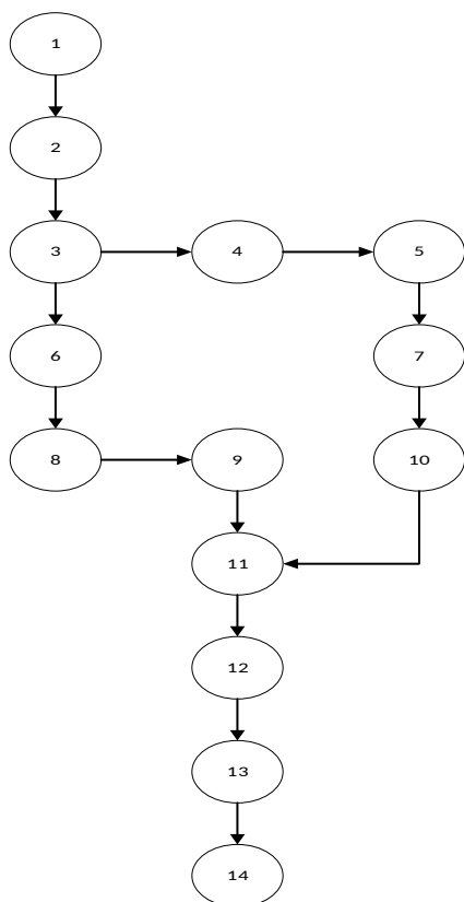
Gambar 4.11 Flowgraph Naive Bayes
