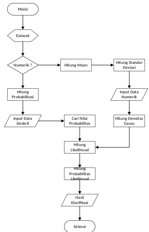
Gambar 4.10 Flowchart Naive Bayes Pesan
