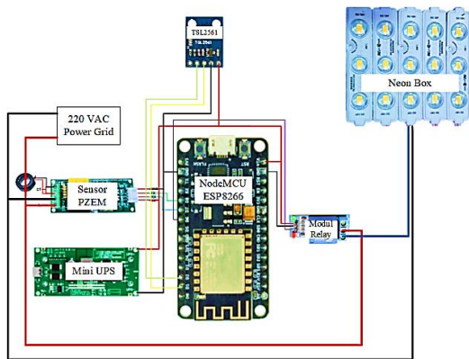
Figure 1. Full System Wiring Diagram
