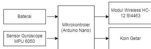
Gambar 7 Blok Diagram Alat
