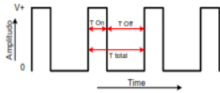
Gambar 1: Sinyal PWM
