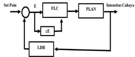
Gambar 6: Blok Diagram Kontrol
