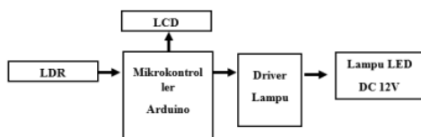
Gambar 5: Diagram Blok sistem
