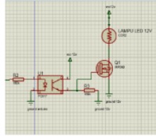
Gambar 8: Driver lampu
