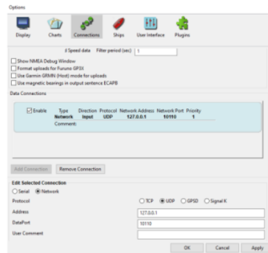
Gambar 12. Pengaturan Connections OpenCPN
