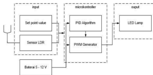
Figure 5. PID dan PWM control system
