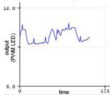
Figure 10. Graph of Signal Coefficient Kp (0.1)
