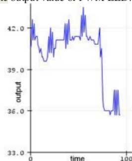
Figure 11. Graph of Signal Coefficient Kp (0.3)
