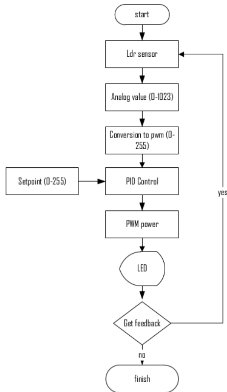
Figure 4. PID dan PWM feedback control flowchart
