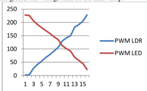
Figure 9. Comparison Graph of Input Value (PWM LDR) and Output Value (PWM LED)
