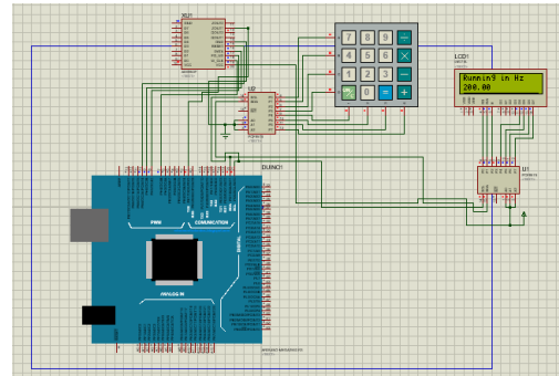
Figure. 8 simulations using a frequency of 200 Hz
