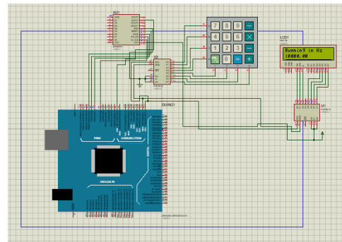
Figure. 9 simulations using a frequency of 10 kHz
