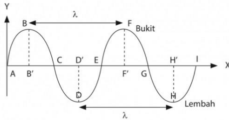
Figure.1 Transverse Waves
