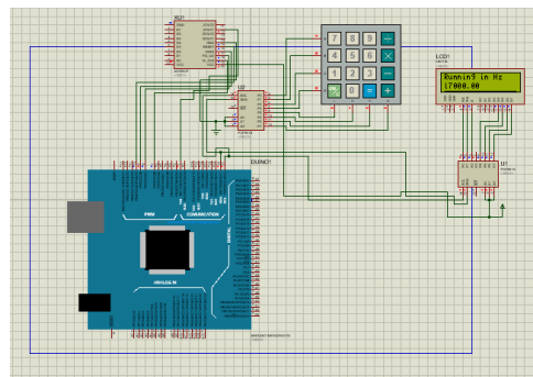
Figure. 10 simulations using a frequency of 17 kHz
