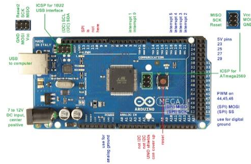
Figure. 3 Arduino mega 2560
