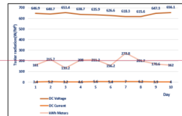
Figure 6. Average data of voltage and current 10 days
