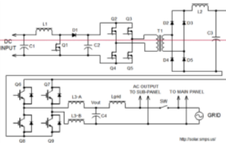
Figure 1. GTI Inverter Circuit
