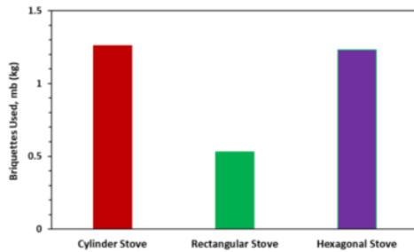
Figure 8. Total mass of burnt briquettes to variations in the shape of a clay stove
