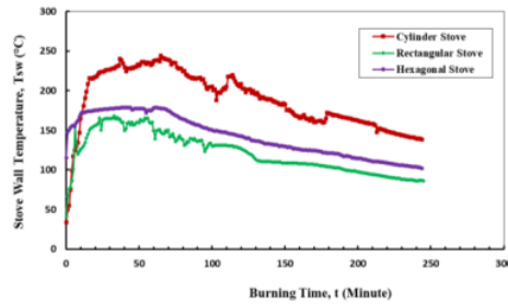
Figure 6. History of Stove Wall Temperature
