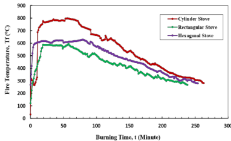
Figure 5. History of Fire Temperature
