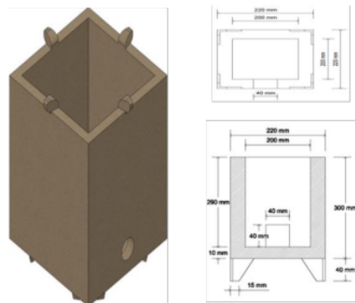
Figure 2. A Rectangular Stove with Dimensions
