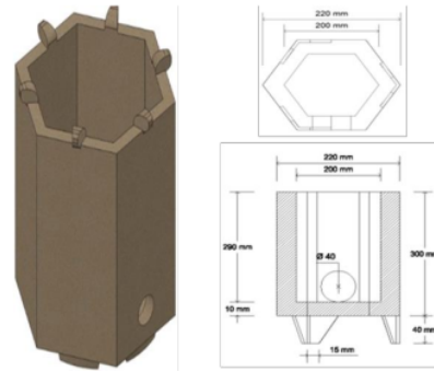
Figure 3. Hexagonal Stove with Dimensions
