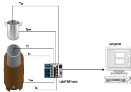
Figure 4. Experimental Installation
