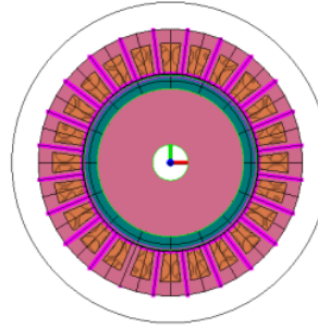
Figure 2. PMSG 24S16P modeling
