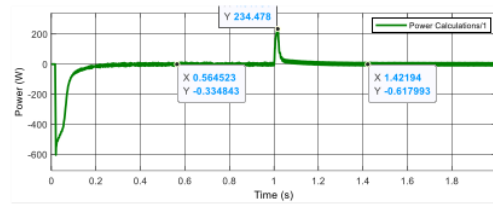
Figure 11. Battery power (supporting storage) scope result
