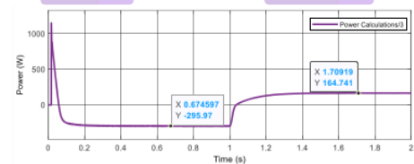
Figure 10. Supercapacitor power (main storage) scope result
