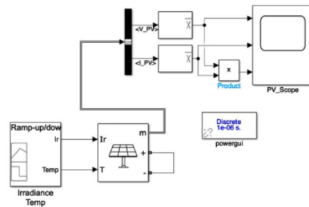
Figure 2. Plant testing short circuit using Simulink
