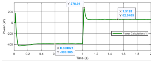
Figure 8. Battery power (main storage) scope result
