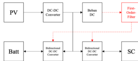
Figure 7. Schematic diagram
