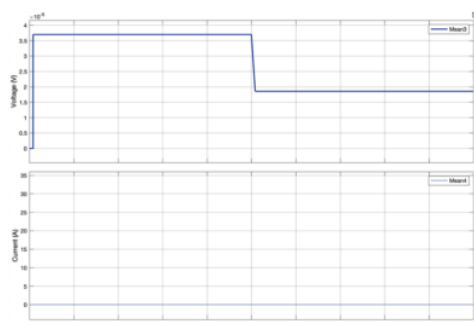
Figure 5. Plant testing short circuit result
