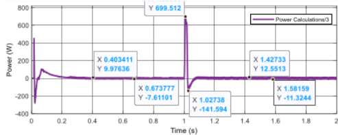
Figure 9. Supercapacitor power (supporting storage) scope result
