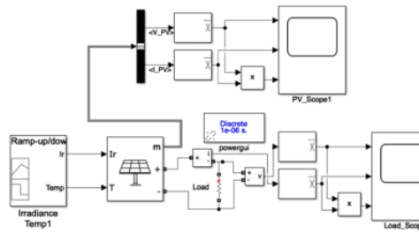
Figure 4. Plant testing short circuit using Simulink
