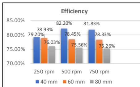
Gambar 12. Efficiency Diagram
