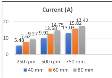
Figure 7. Current Diagram
