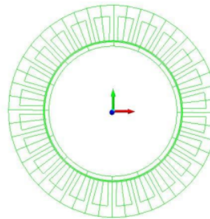
Figure 2. Line on PMSG 24s16p
