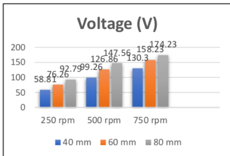
Figure 8. Voltage Diagram
