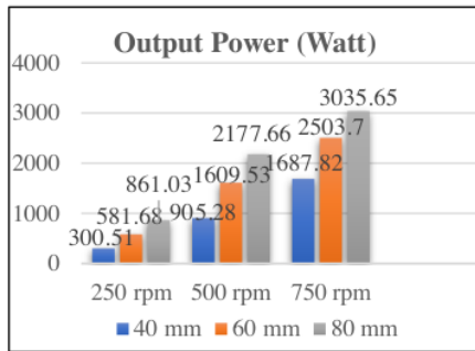
Figure 11. Output Power Diagram
