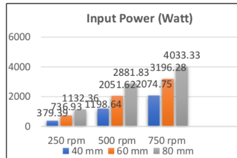
Figure 10. Input Power Diagram
