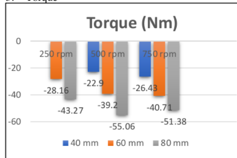
Figure 9. Torque Diagram
