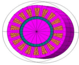
Figure 3. Permanent Magnet Synchronous Generator 18 Slots 16 Poles
