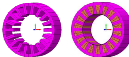
Figure 2. Stator material Carpenter: Silicon Steel and winding copper
