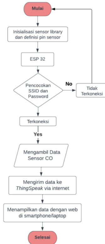
Figure 4. Flowchart of carbon monoxide (CO) measurement system
