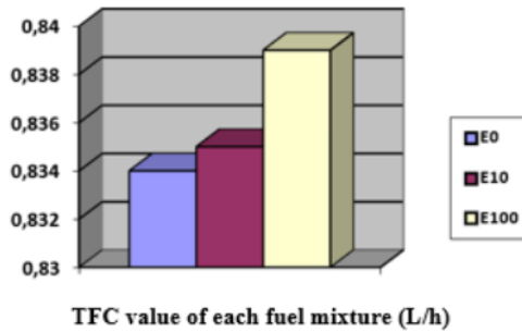
Figure 5. Graph of TFC Comparison of Bioethanol Pineapple Skin Waste on Various Fuels (E0,E10,E100)
