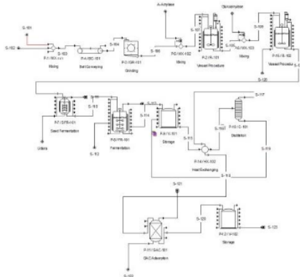
Figure 2. Simulation of a Pineapple Skin Waste Bioethanol Reactor Using the Superpro
