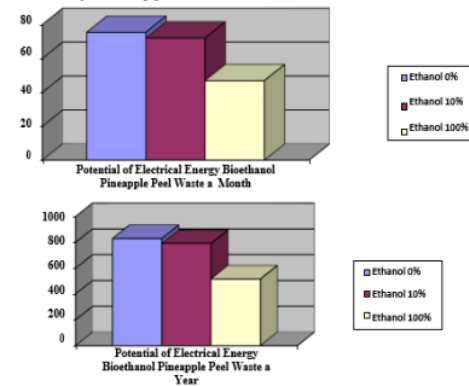
Figure 3 Graph of Potential Electrical Energy that Can be Generated by Pineapple Skin Waste Bioethanol with Various Fuel Mixtures/Month and/Year
