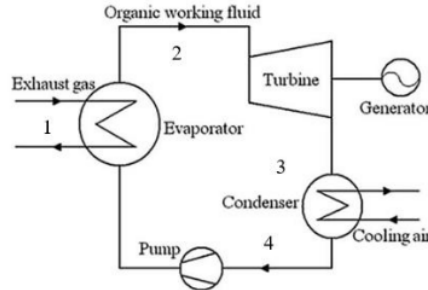
Figure 2. Organic Rankine Cycle Scheme [15]
