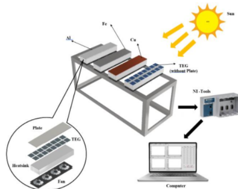
Figure 1. The scheme of Test Installation
