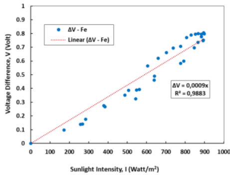
Figure 7. Linear correlation of voltage on the iron absorber TEMs module with solar intensity
