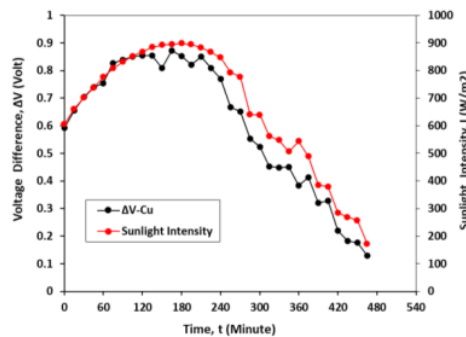
Figure 4. The pattern of changes in the voltage of the TEMs module with respect to the time of increasing solar intensity
